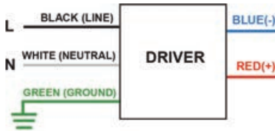
WIRING DIAGRAM
