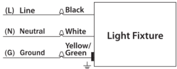
Wiring diagram
