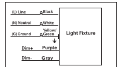
Wiring Diagram (Dimming wire optional)
