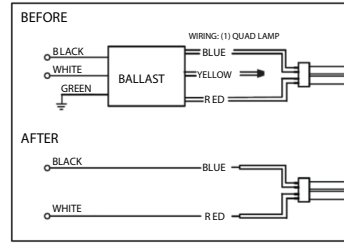
Figure 3: Retrofit with one lamp (G24q Base)
