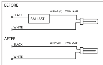
Figure 1: Retrofit with one lamp (GX23 Base)
